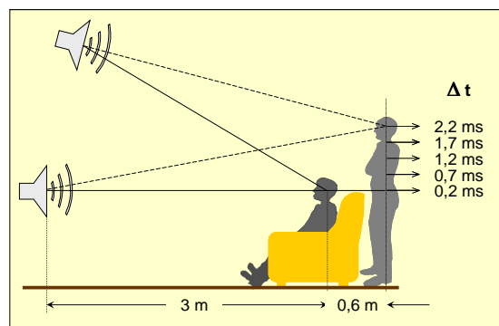
Figure 4: Delay differences occurring in listening positions beyond the sweet spot
